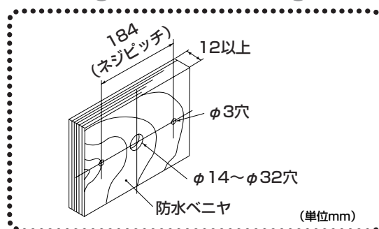
● ● ● 裏うち板参考寸法図 ● ● ●
